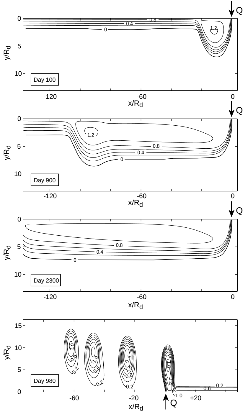
Fig. 7. The same as the zero potential vorticity case ( Fig. 6 ) except that the outflow's potential vorticity is now finite ( H_p = 1100 m; H = 470 m). It shows that the difference between the two is minimal.
